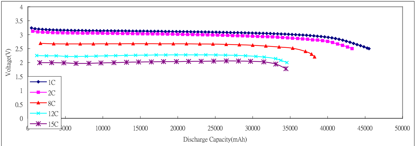
(25°C) 42Ah Cylindrical (World PAT.) or Prismatic (World PAT.) Cell PAT. C-LiFePO 4
