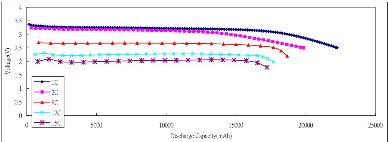
(25°C) 22Ah Cylindrical (World PAT.) or Prismatic (World PAT.) Cell PAT. C-LiFePO 4
