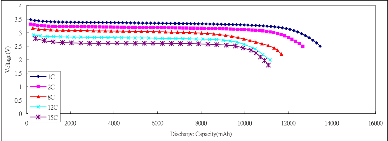
(25°C) 12Ah Cylindrical (World PAT.) or Prismatic (World PAT.) Cell PAT. C-LiFePO 4
