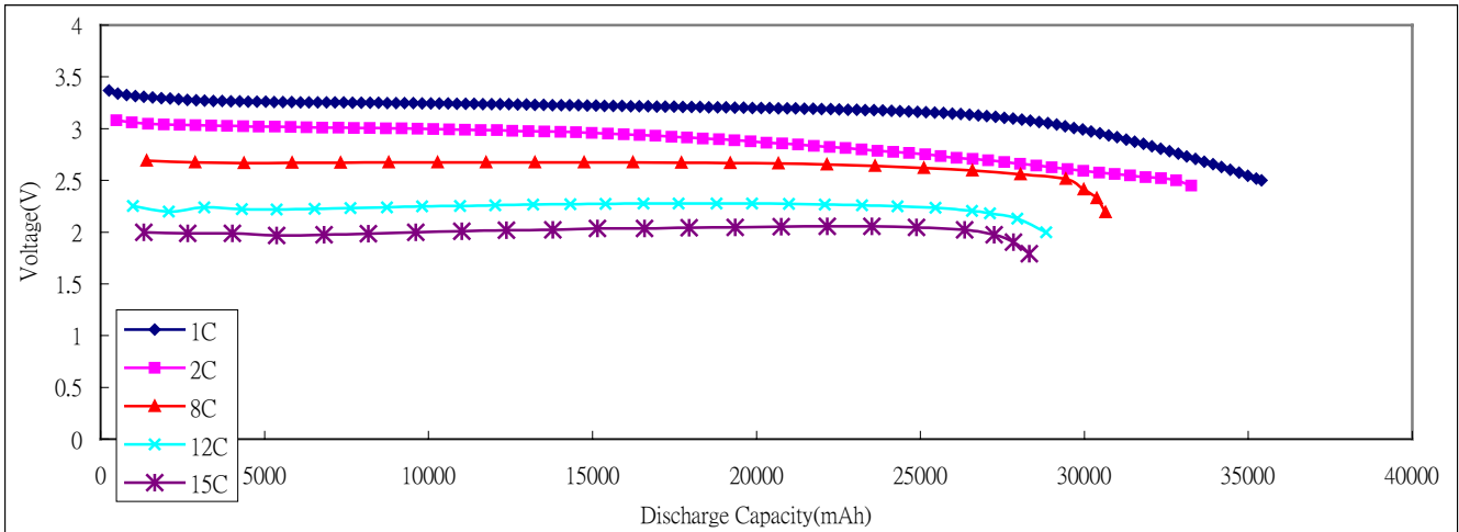
(25°C) 35Ah Cylindrical (World PAT.) or Prismatic (World PAT.) Cell PAT. C-LiFePO 4
