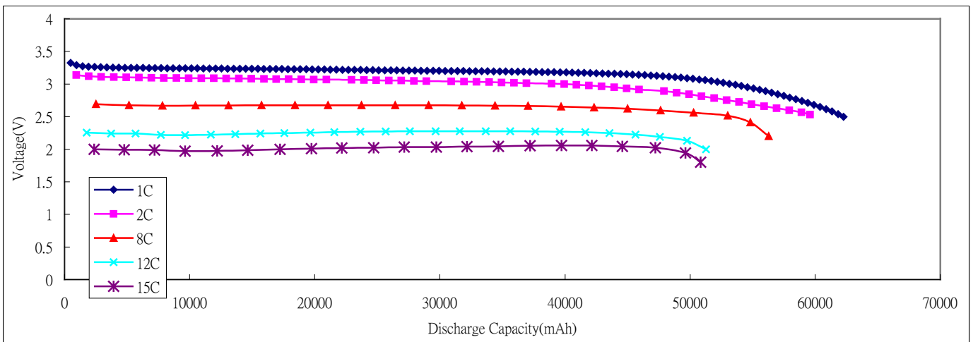
(25°C) 60Ah Cylindrical (World PAT.) or Prismatic (World PAT.) Cell PAT. C-LiFePO 4
